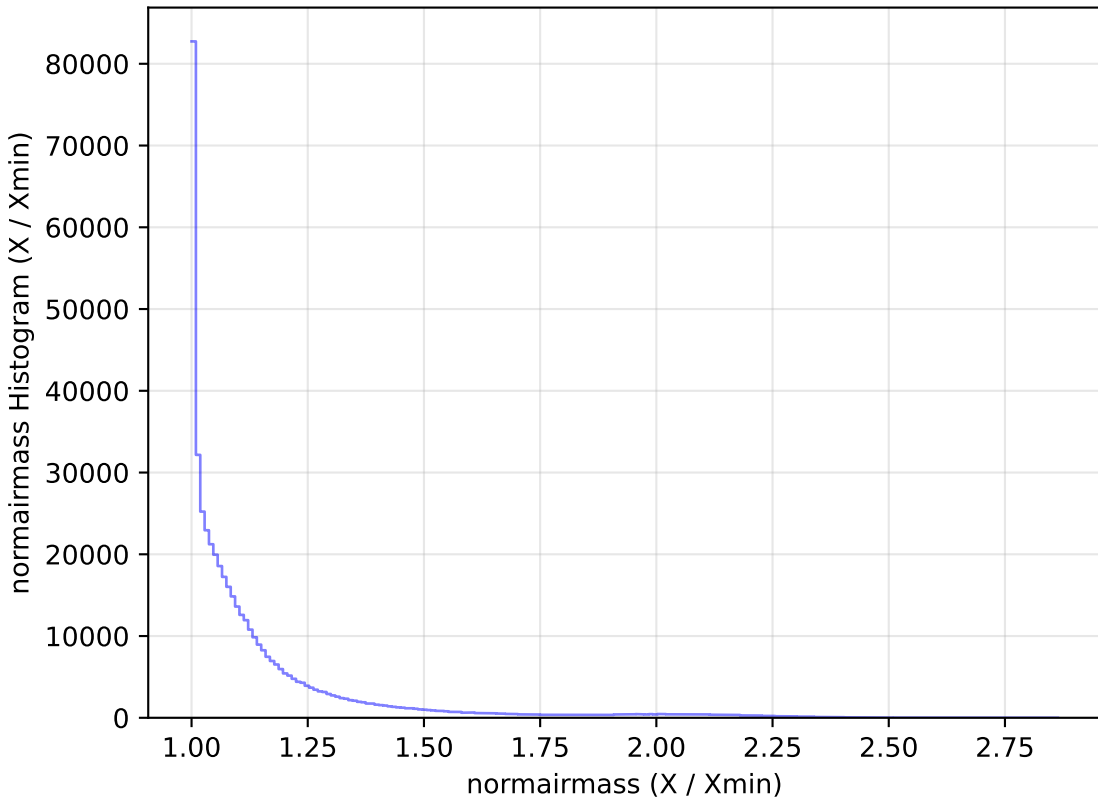
ddf_loaded_fl4_v3.4_10yrs All sky r band: normairmass Histogram
