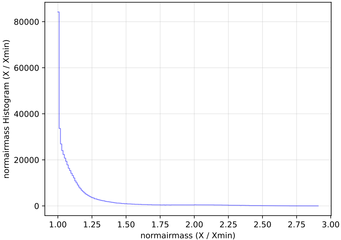
ddf_loaded_fl4_v3.4_10yrs All sky i band: normairmass Histogram
