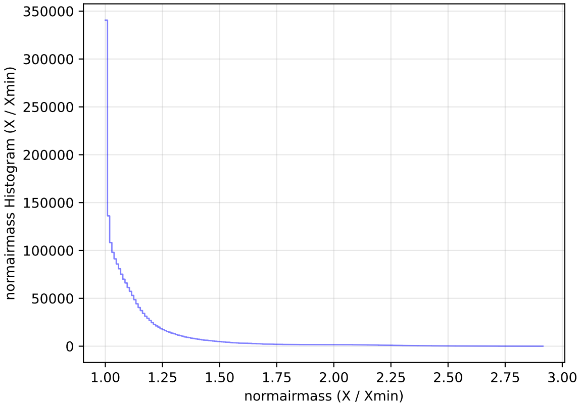
ddf_loaded_fl4_v3.4_10yrs All sky all bands: normairmass Histogram
