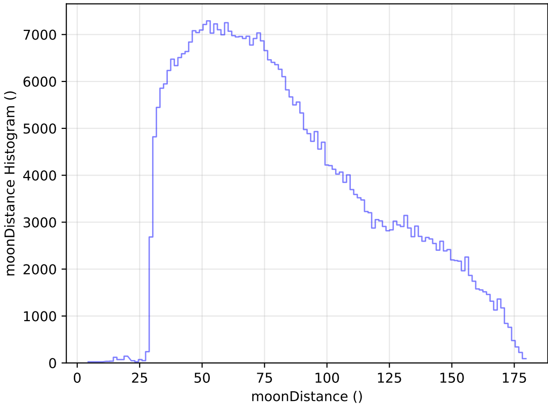
ddf_loaded_fl4_v3.4_10yrs WFD z band: moonDistance Histogram
