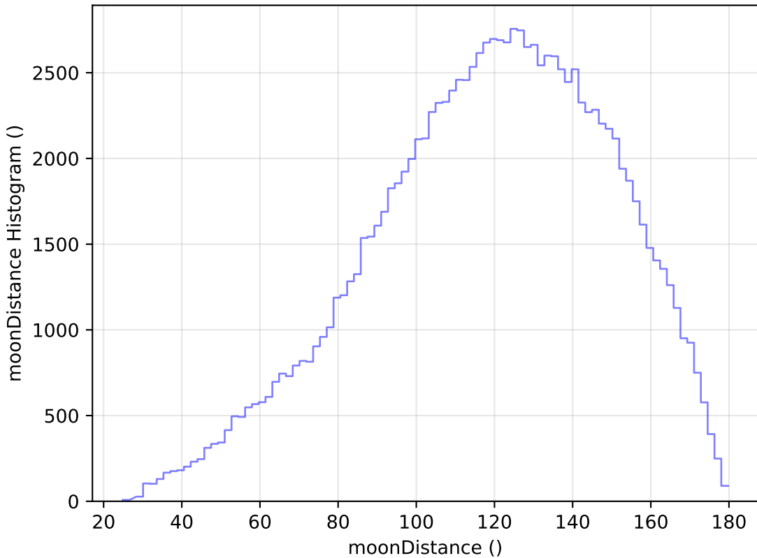
ddf_loaded_fl4_v3.4_10yrs WFD u band: moonDistance Histogram
