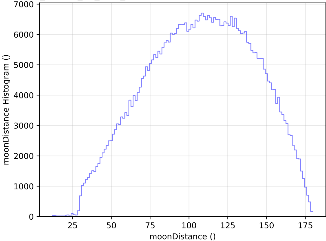
ddf_loaded_fl4_v3.4_10yrs WFD r band: moonDistance Histogram
