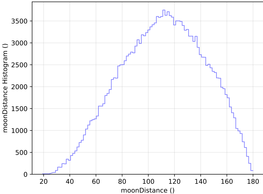
ddf_loaded_fl4_v3.4_10yrs WFD g band: moonDistance Histogram
