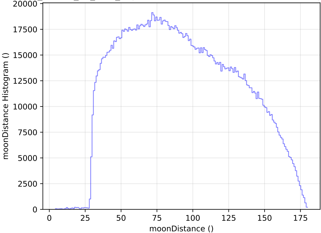
ddf_loaded_fl4_v3.4_10yrs WFD all bands: moonDistance Histogram
