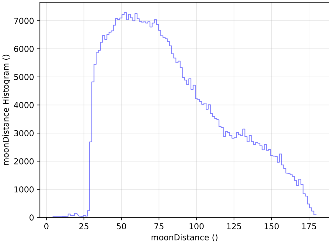
ddf_loaded_fl4_v3.4_10yrs All sky z band: moonDistance Histogram
