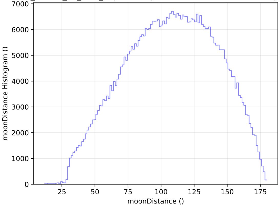
ddf_loaded_fl4_v3.4_10yrs All sky r band: moonDistance Histogram
