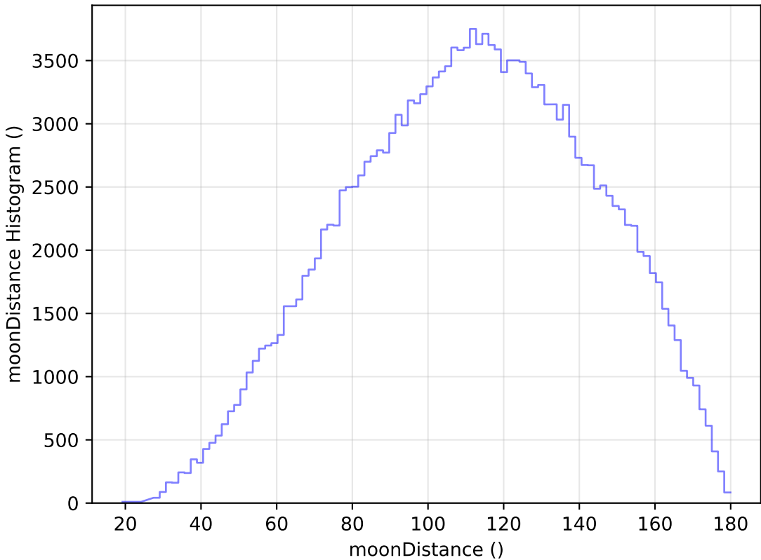
ddf_loaded_fl4_v3.4_10yrs All sky g band: moonDistance Histogram
