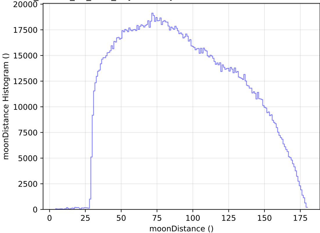
ddf_loaded_fl4_v3.4_10yrs All sky all bands: moonDistance Histogram
