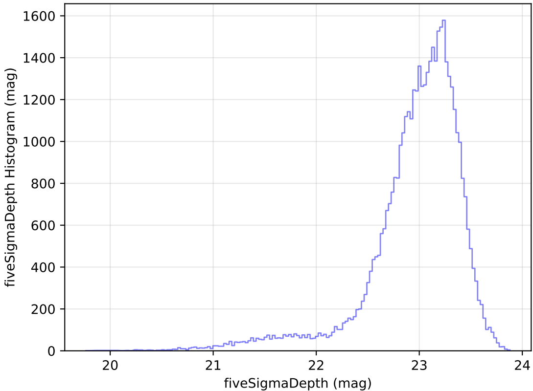
ddf_loaded_fl4_v3.4_10yrs Yr 1 z band: fiveSigmaDepth Histogram
