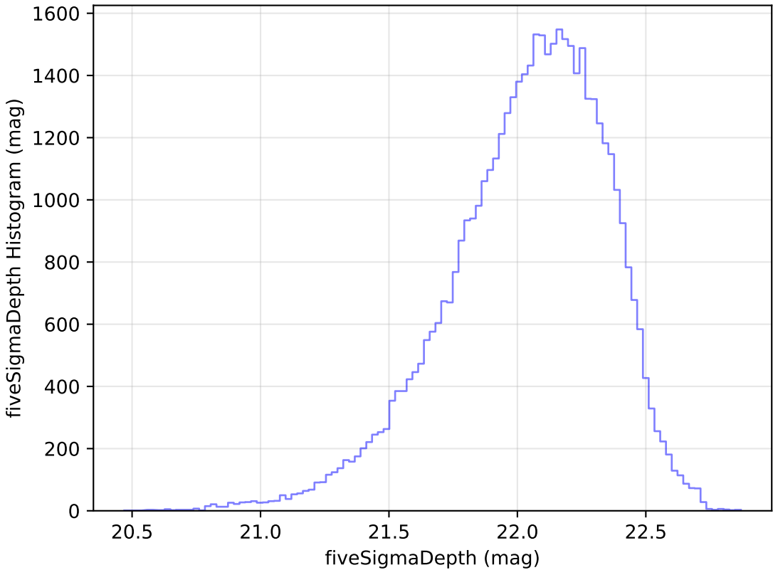
ddf_loaded_fl4_v3.4_10yrs Yr 1 y band: fiveSigmaDepth Histogram
