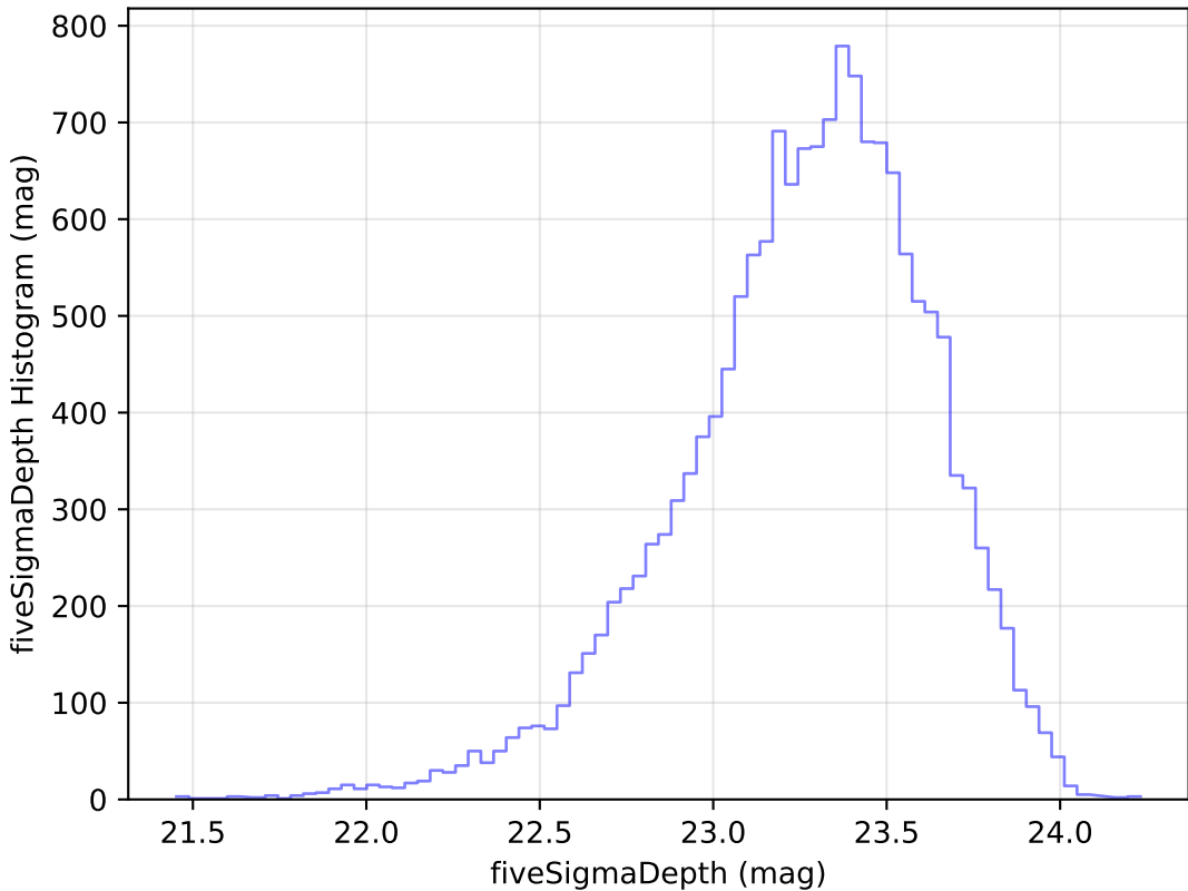
ddf_loaded_fl4_v3.4_10yrs Yr 1 u band: fiveSigmaDepth Histogram
