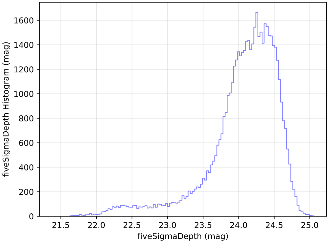
ddf_loaded_fl4_v3.4_10yrs Yr 1 r band: fiveSigmaDepth Histogram
