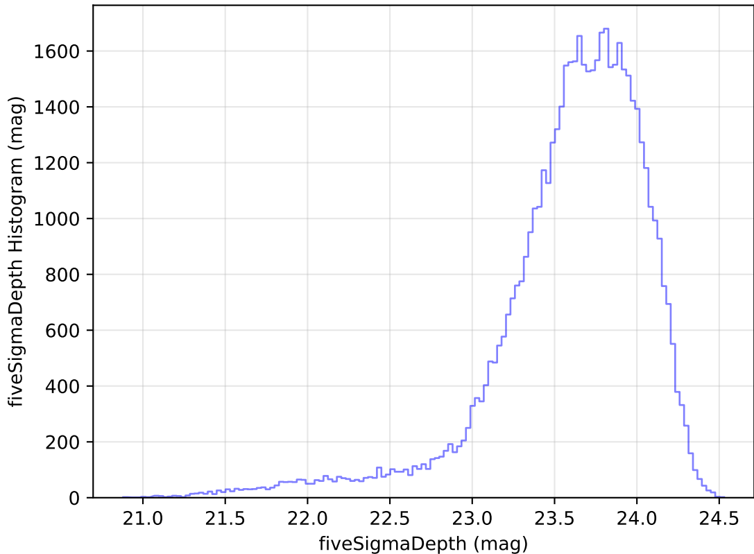
ddf_loaded_fl4_v3.4_10yrs Yr 1 i band: fiveSigmaDepth Histogram
