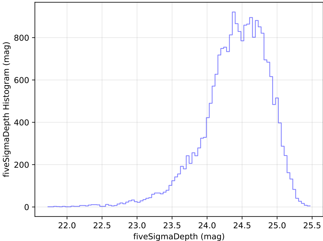
ddf_loaded_fl4_v3.4_10yrs Yr 1 g band: fiveSigmaDepth Histogram
