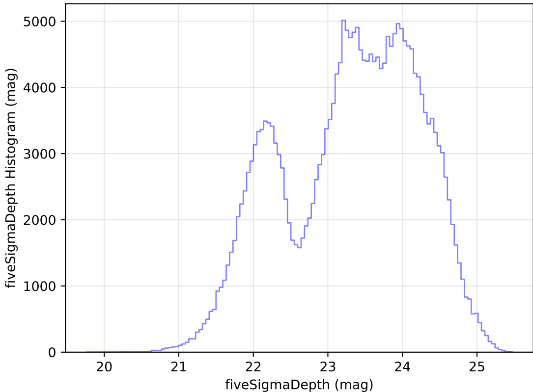
ddf_loaded_fl4_v3.4_10yrs Yr 1 all bands: fiveSigmaDepth Histogram
