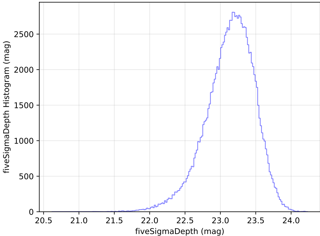
ddf_loaded_fl4_v3.4_10yrs WFD u band: fiveSigmaDepth Histogram
