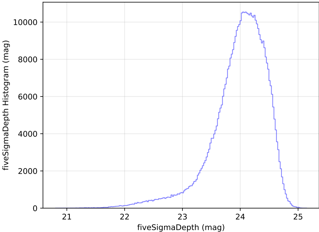
ddf_loaded_fl4_v3.4_10yrs WFD r band: fiveSigmaDepth Histogram
