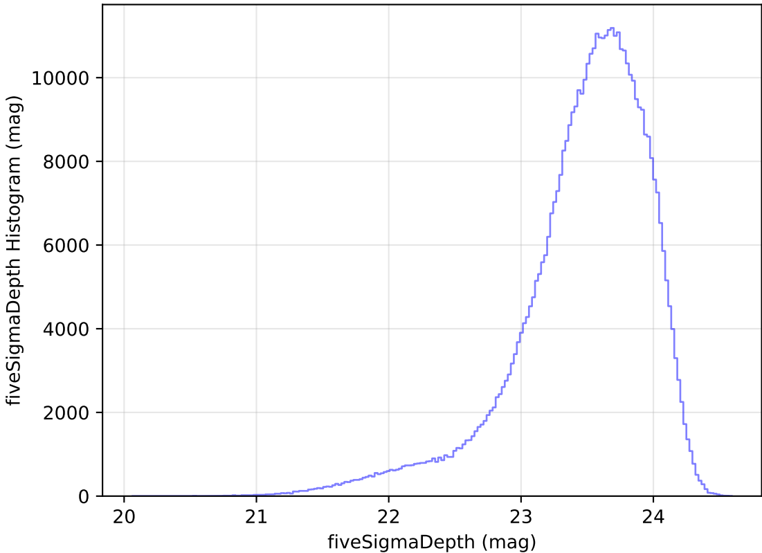
ddf_loaded_fl4_v3.4_10yrs WFD i band: fiveSigmaDepth Histogram
