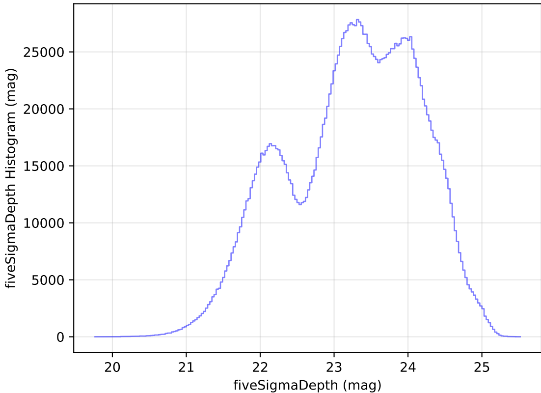
ddf_loaded_fl4_v3.4_10yrs WFD all bands: fiveSigmaDepth Histogram
