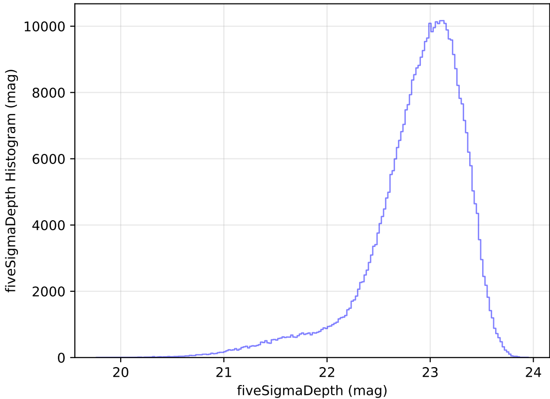
ddf_loaded_fl4_v3.4_10yrs All sky z band: fiveSigmaDepth Histogram
