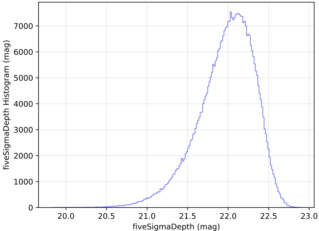
ddf_loaded_fl4_v3.4_10yrs All sky y band: fiveSigmaDepth Histogram
