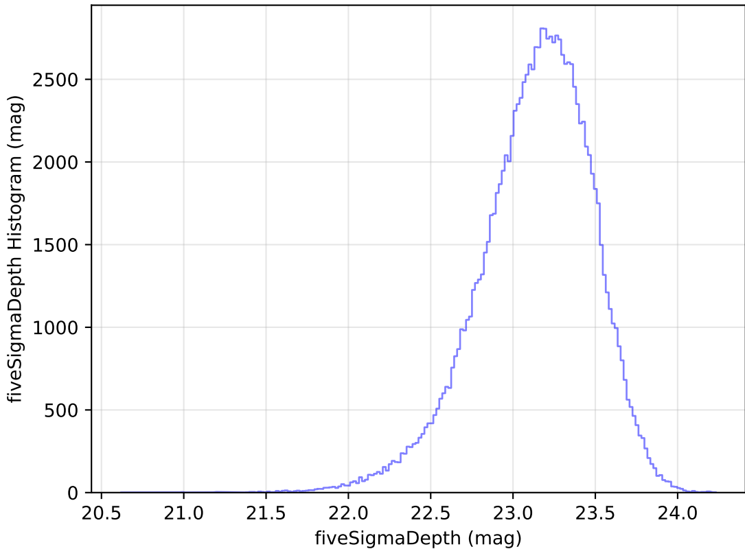
ddf_loaded_fl4_v3.4_10yrs All sky u band: fiveSigmaDepth Histogram
