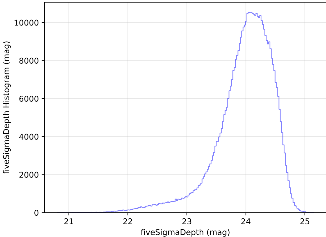
ddf_loaded_fl4_v3.4_10yrs All sky r band: fiveSigmaDepth Histogram
