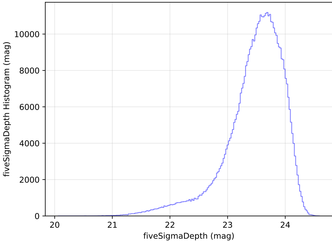
ddf_loaded_fl4_v3.4_10yrs All sky i band: fiveSigmaDepth Histogram
