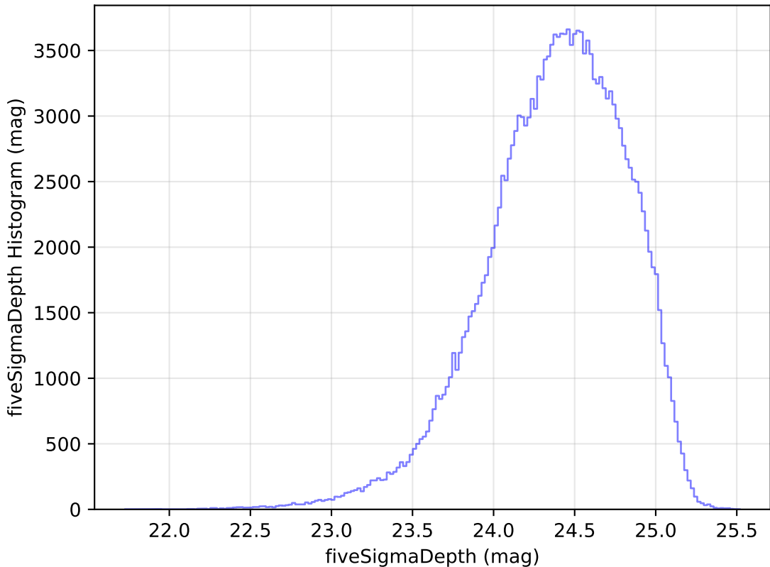
ddf_loaded_fl4_v3.4_10yrs All sky g band: fiveSigmaDepth Histogram
