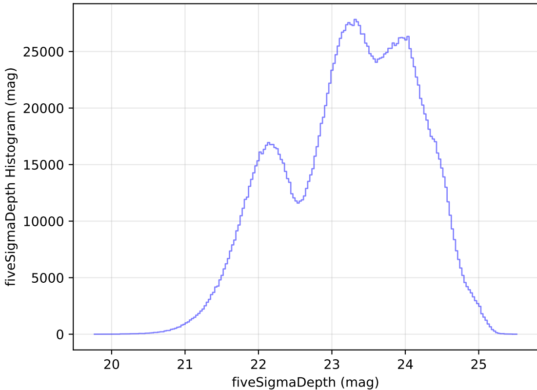
ddf_loaded_fl4_v3.4_10yrs All sky all bands: fiveSigmaDepth Histogram
