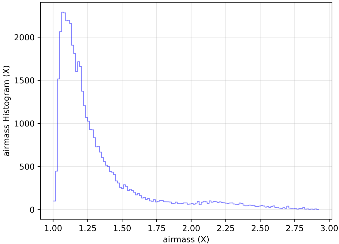
ddf_loaded_fl4_v3.4_10yrs Yr 1 z band: airmass Histogram
