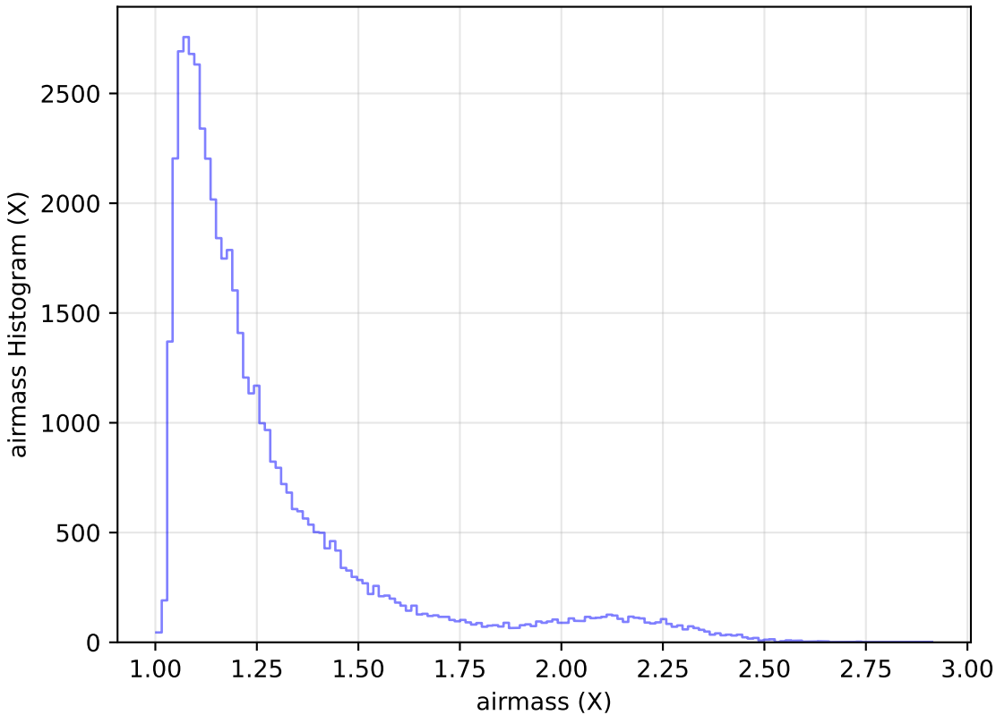
ddf_loaded_fl4_v3.4_10yrs Yr 1 r band: airmass Histogram
