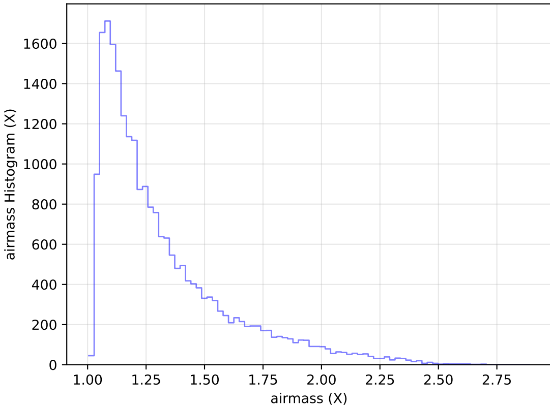
ddf_loaded_fl4_v3.4_10yrs Yr 1 g band: airmass Histogram
