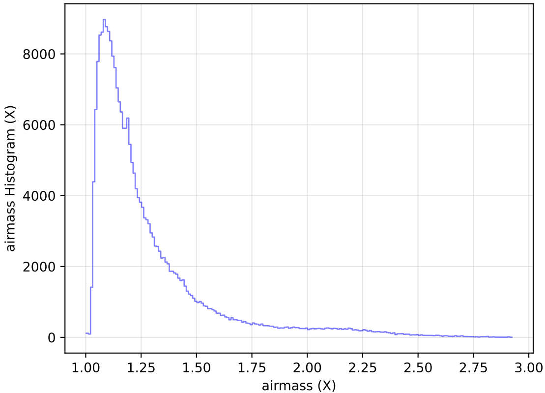
ddf_loaded_fl4_v3.4_10yrs Yr 1 all bands: airmass Histogram
