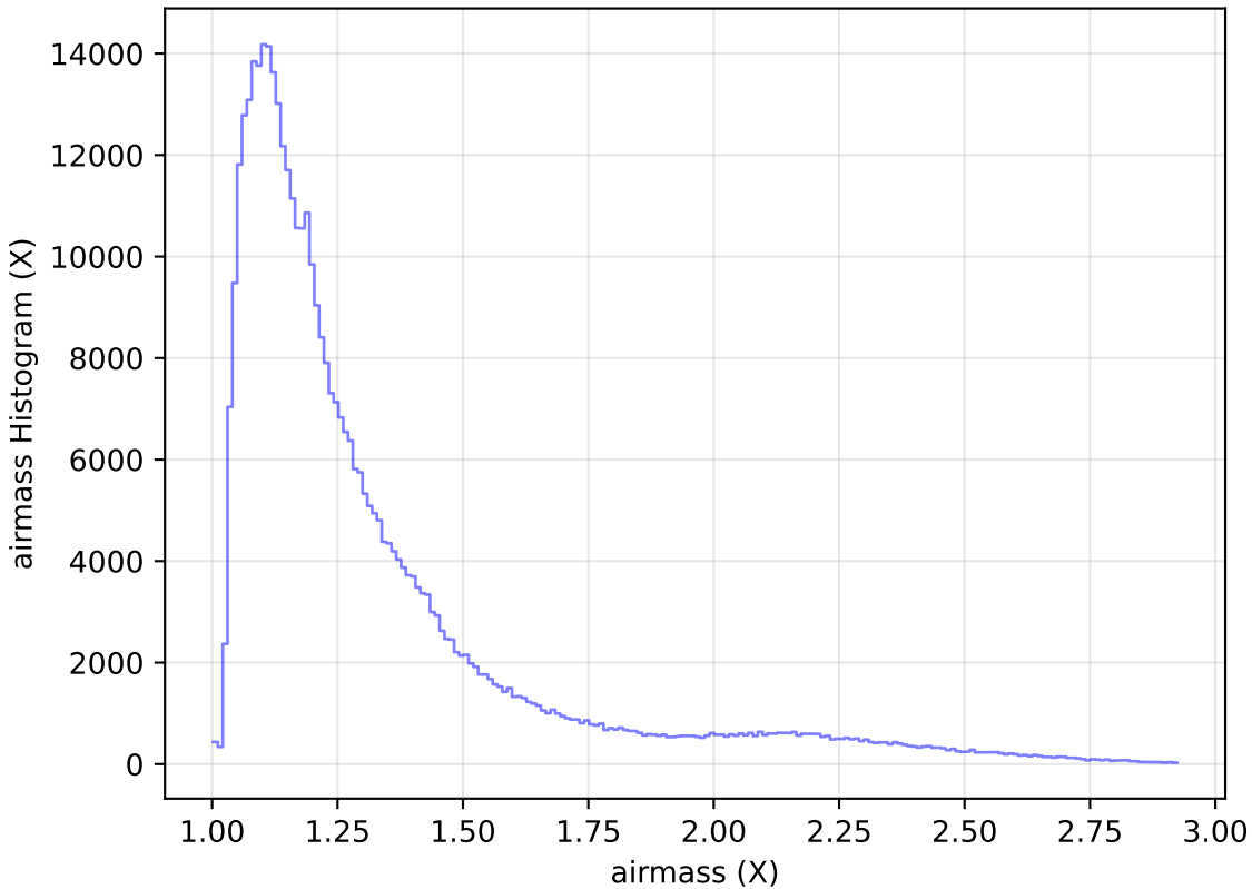
ddf_loaded_fl4_v3.4_10yrs WFD z band: airmass Histogram
