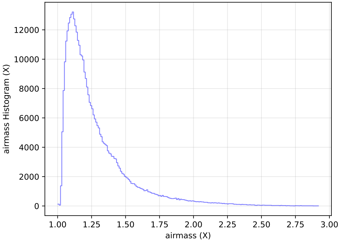
ddf_loaded_fl4_v3.4_10yrs WFD y band: airmass Histogram
