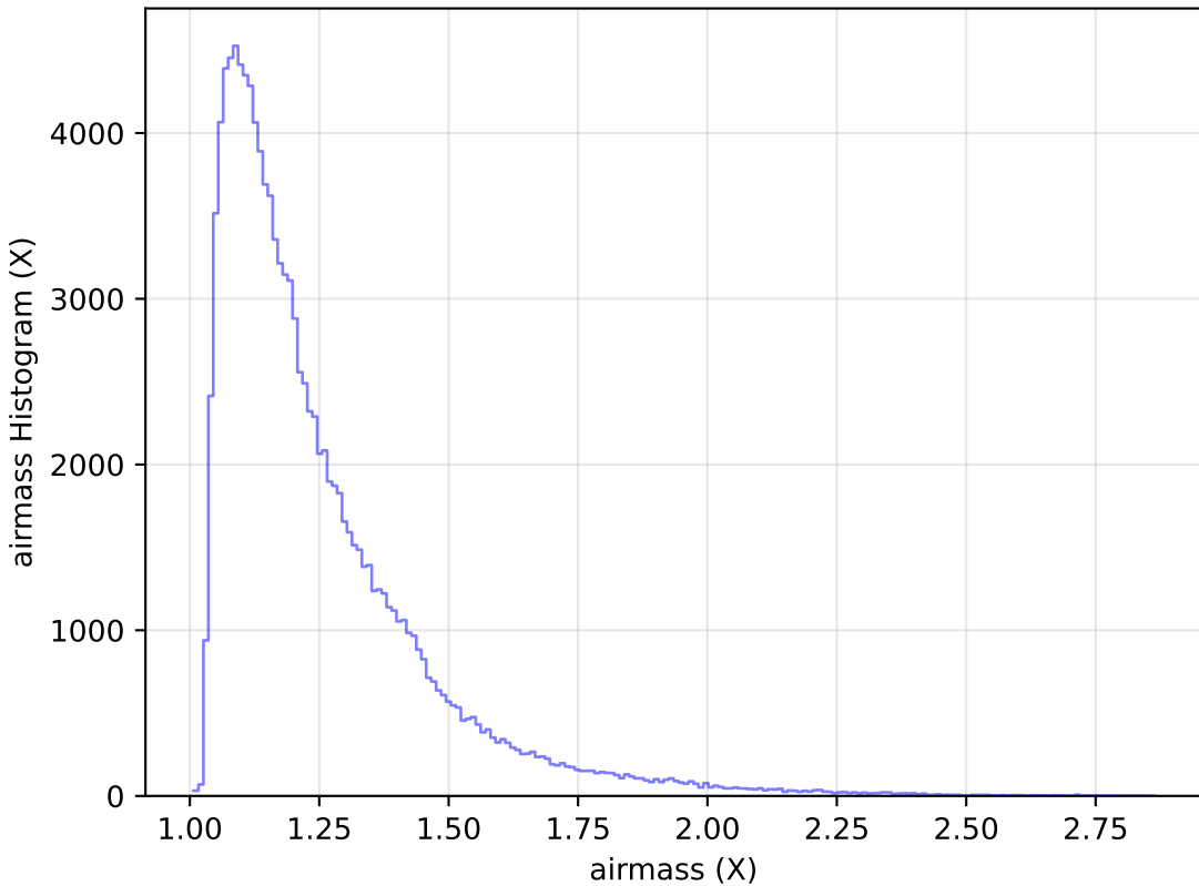
ddf_loaded_fl4_v3.4_10yrs WFD u band: airmass Histogram
