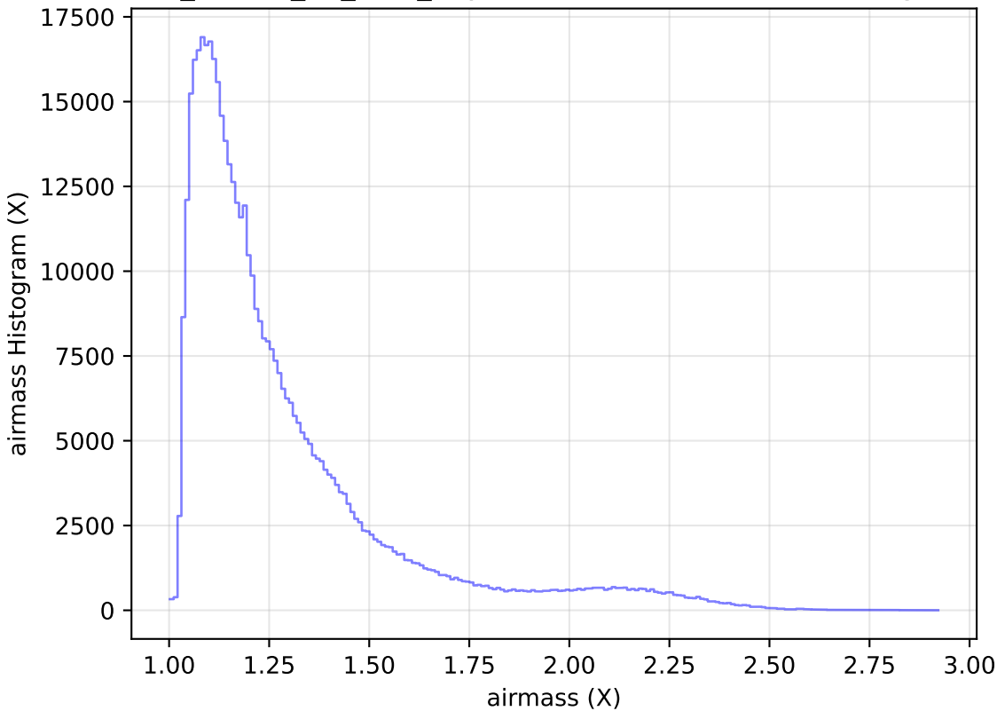
ddf_loaded_fl4_v3.4_10yrs WFD r band: airmass Histogram
