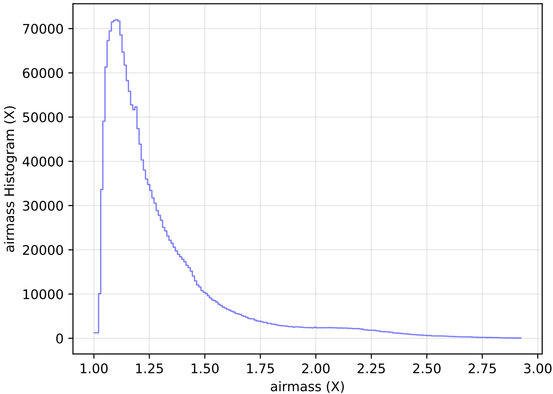
ddf_loaded_fl4_v3.4_10yrs WFD all bands: airmass Histogram
