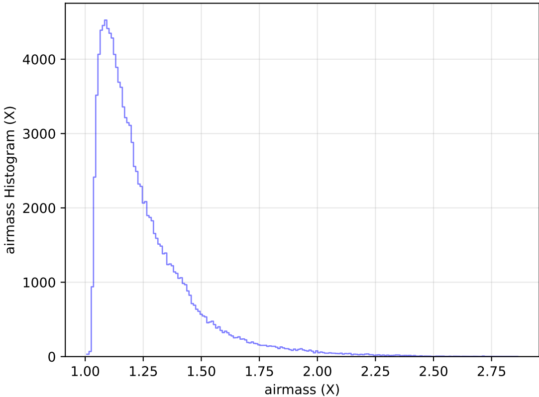
ddf_loaded_fl4_v3.4_10yrs All sky u band: airmass Histogram
