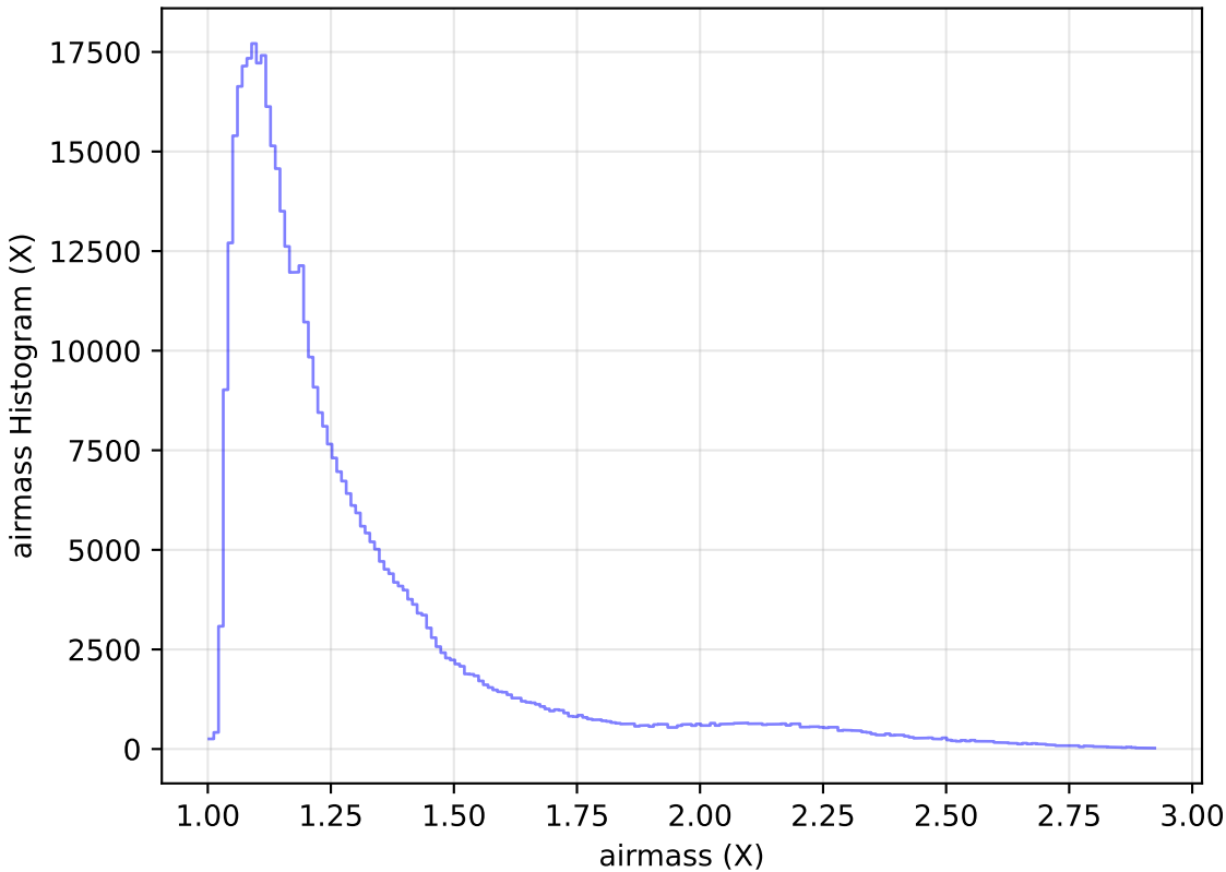
ddf_loaded_fl4_v3.4_10yrs All sky i band: airmass Histogram
