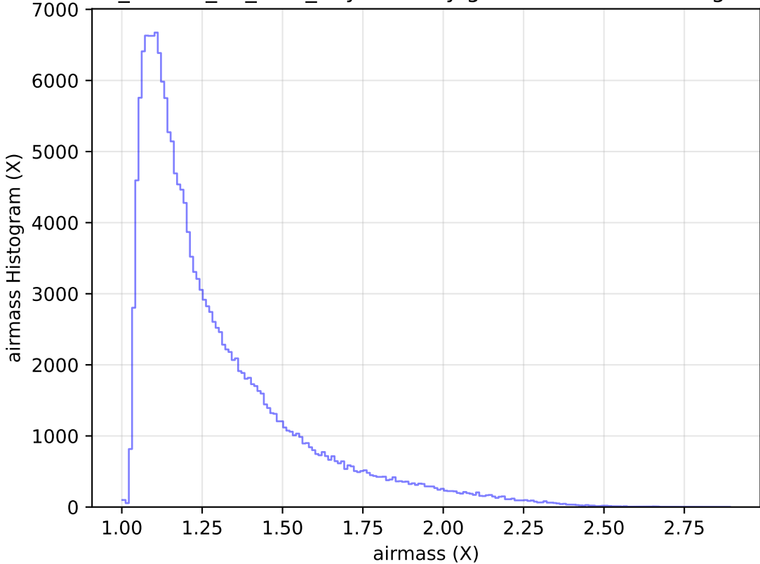
ddf_loaded_fl4_v3.4_10yrs All sky g band: airmass Histogram
