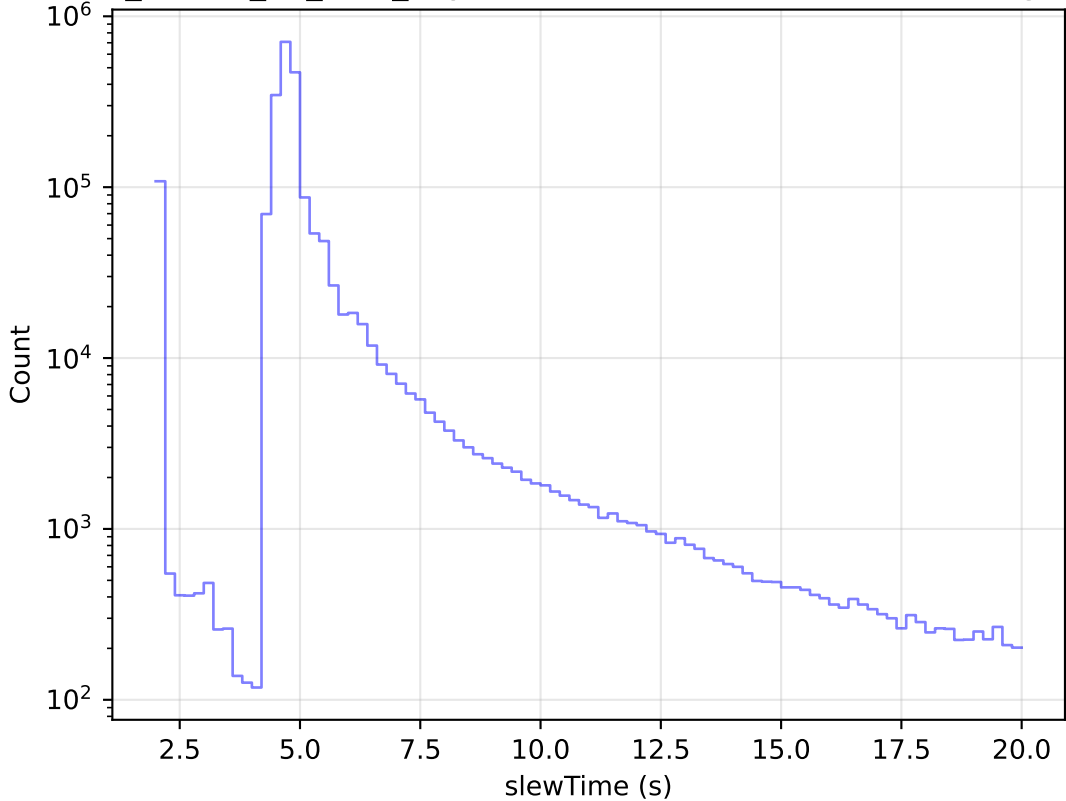
ddf_loaded_fl4_v3.4_10yrs All visits: Zoom Slew Time Histogram
