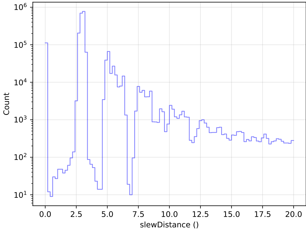
ddf_loaded_fl4_v3.4_10yrs All visits: Zoom Slew Distance Histogram
