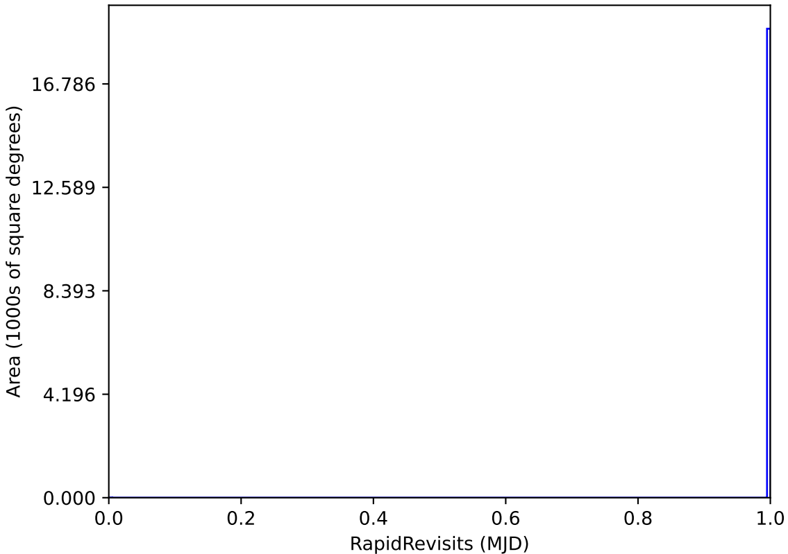
ddf_loaded_fl4_v3.4_10yrs WFD: RapidRevisits
