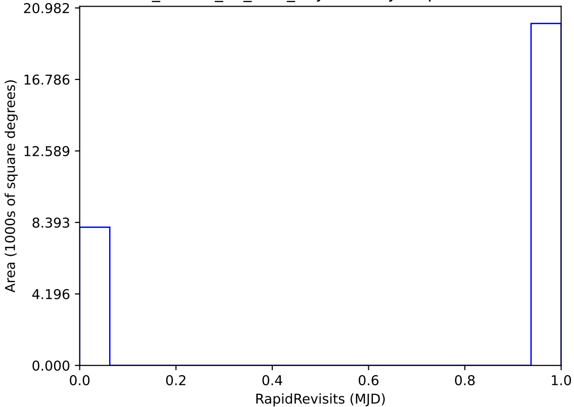
ddf_loaded_fl4_v3.4_10yrs All sky: RapidRevisits
