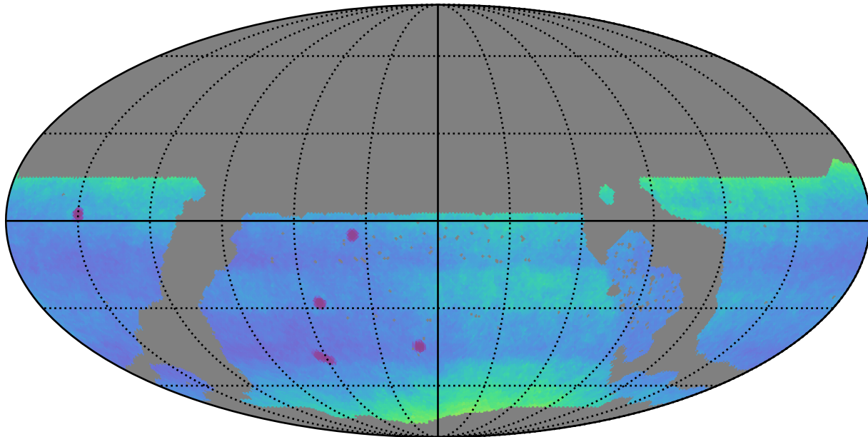
ddf_loaded_fl4_v3.4_10yrs WFD: Proper Motion Uncert @ 24.0
