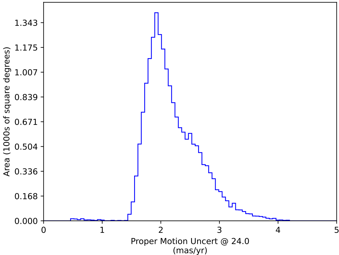
ddf_loaded_fl4_v3.4_10yrs WFD: Proper Motion Uncert @ 24.0
