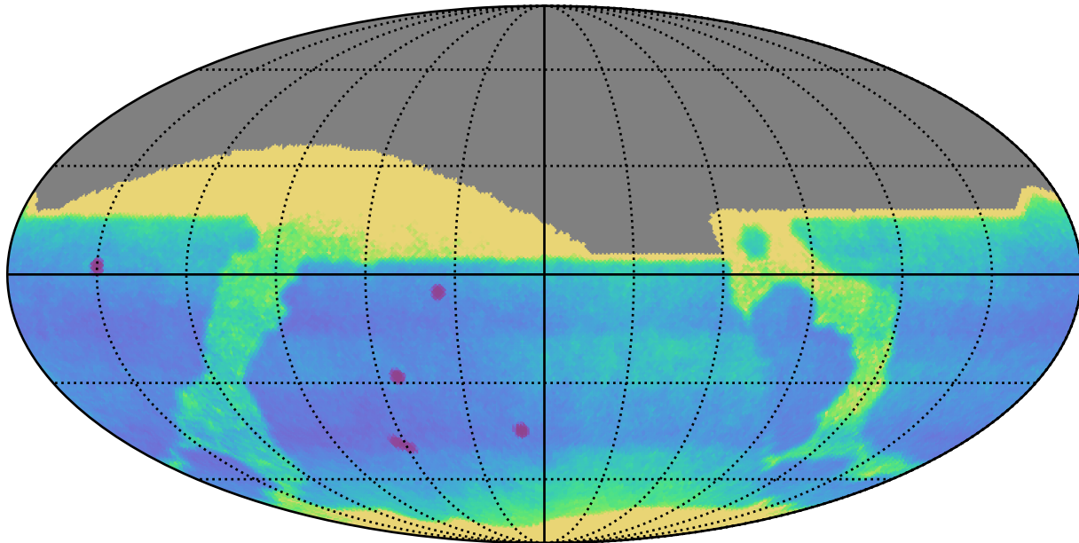
ddf_loaded_fl4_v3.4_10yrs All sky: Proper Motion Uncert @ 24.0
