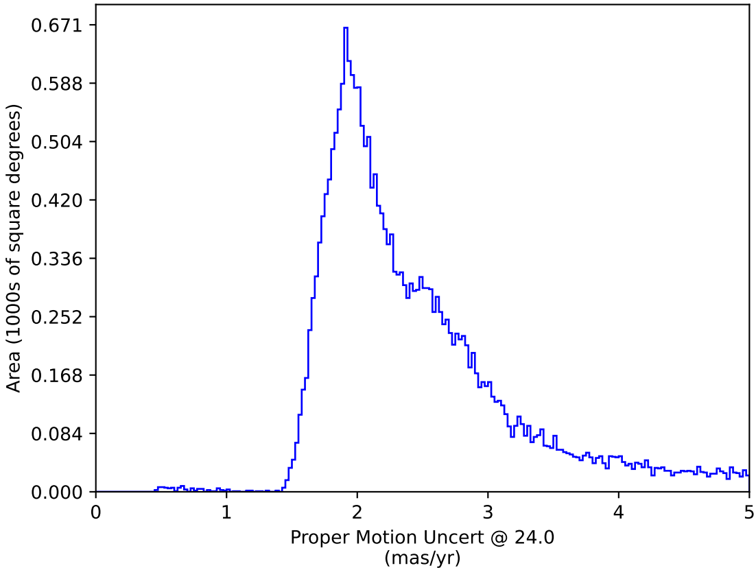
ddf_loaded_fl4_v3.4_10yrs All sky: Proper Motion Uncert @ 24.0
